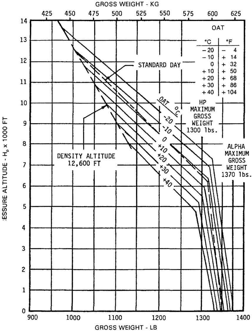
OGE HOVER CEILING VS. GROSS WEIGHT
