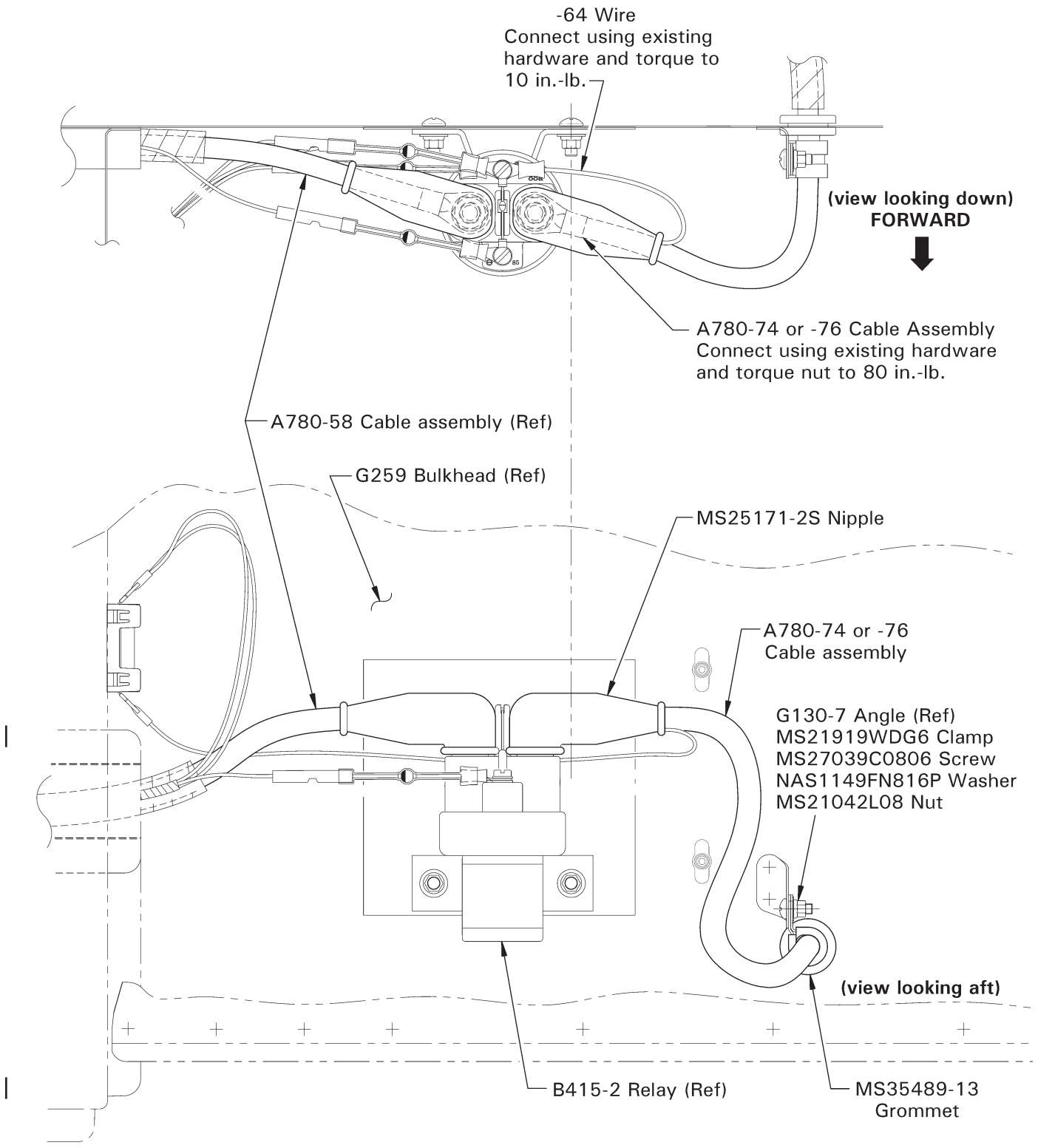
FIGURE 7 Installation of A780 cable assembly with fuse holder (Aft-left seat back removed)
