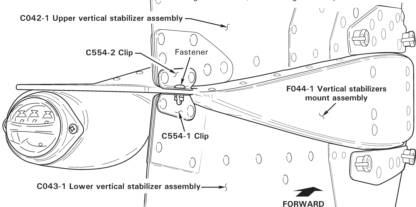
FIGURE 53-7 F004-2 EMPENNAGE ASSEMBLY – TAILCONE ASSEMBLY AFT BULKHEAD
